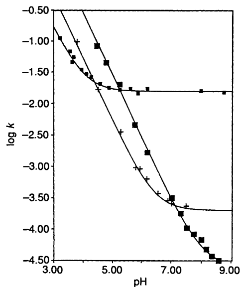
Fig. 1 pH-Dependence of observed rate constants for the disappearance of 1,5-dimethyl-5-(aryloxy)-6-acetylaminocyclohexa-1,3-dienes: (■) 12a , benzoyloxy; (+) 12b , m -nitrobenzoyloxy; (■) 12c , pentafluorobenzoyloxy ( k obs in units of s -1 , at 40 °C and ionic strength 1 mol dm -3 in 8.3% by volume acetonitrile)
