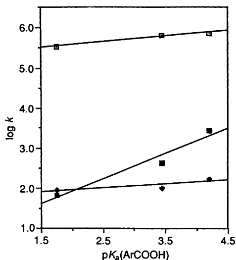
Fig. 2 Dependence of \log k_{\text{H}}(\text{phenol}) (◆), \log k_{\text{H}}(\text{ester}) (■) and \log k_{\text{H}}(\text{Az}) (□) on the pK_a of the aryloxy leaving group. Slopes of the lines are 0.09, 0.63 and 0.13, respectively. Values of k_{\text{H}}(\text{phenol}) and k_{\text{H}}(\text{ester}) have been calculated by multiplying the observed k_{\text{H}} (Table 1) by the fractions of meta -substituted phenol and meta -substituted ester (Table 2), respectively.
